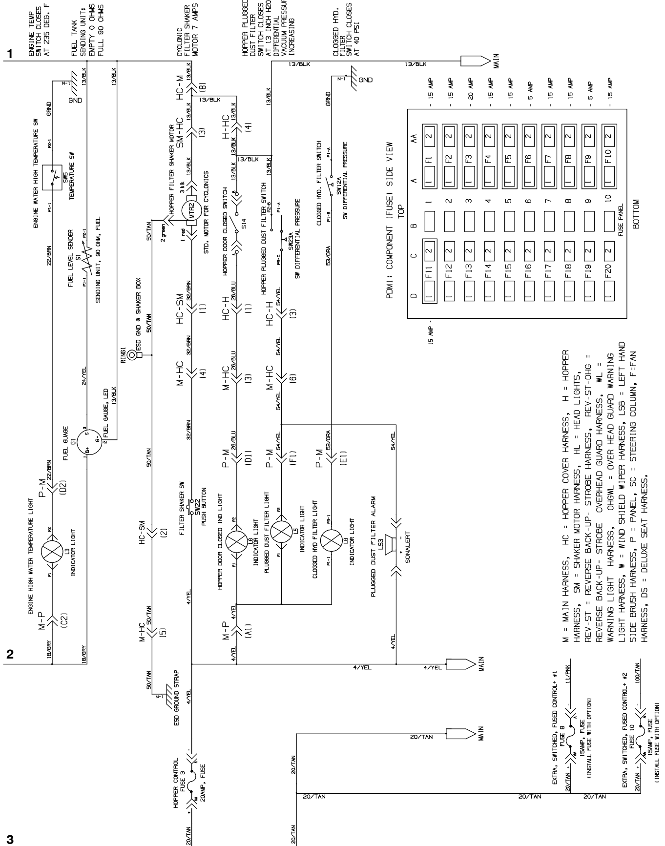
Fig. 42 - Electrical Schematic
