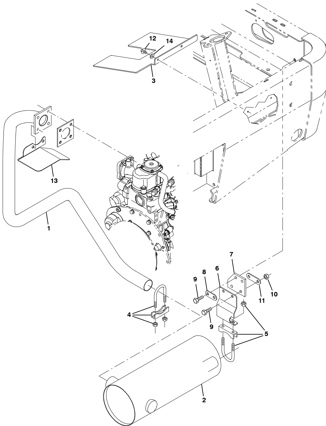
Fig. 18 - Engine Muffler Group
