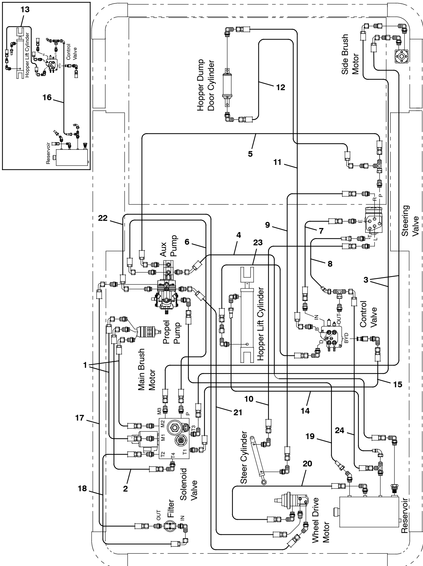
Fig. 39 - Hydraulic Hose Group
