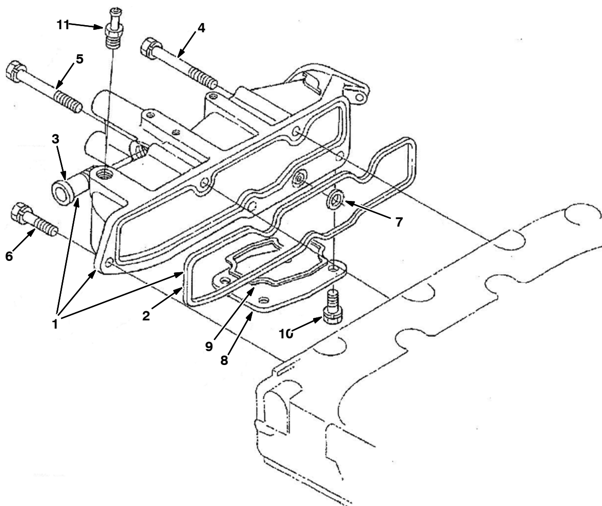
Fig. 26 - Inlet Manifold Group
