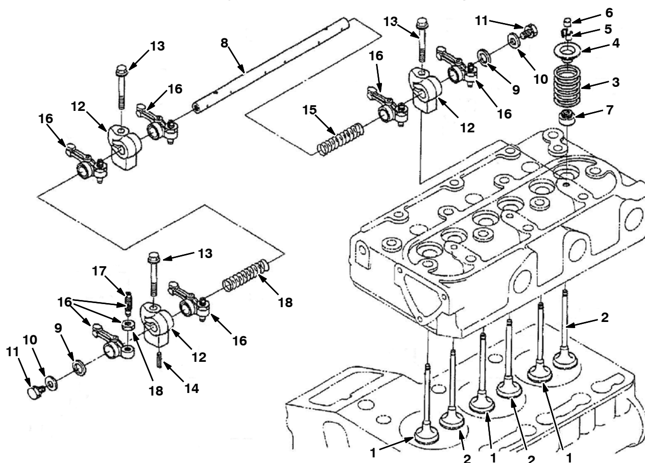
Fig. 24 - Valve and Rocker Arm Group
