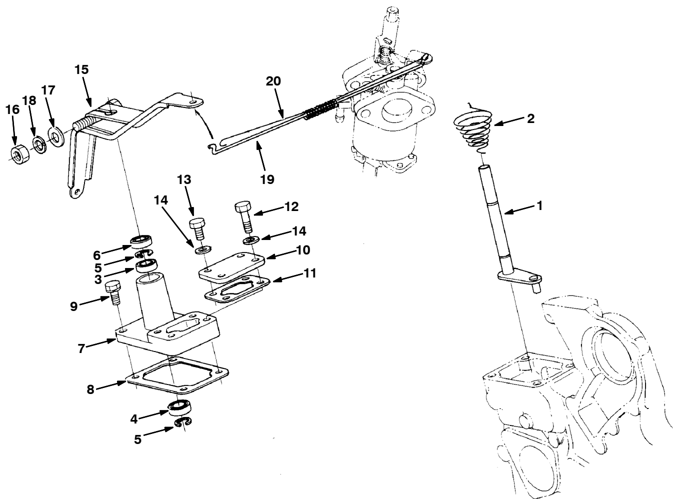
Fig. 13 - Governor Group
