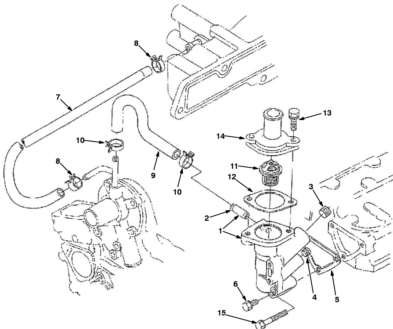
Fig. 20 - Water Flange and Thermostat Group
