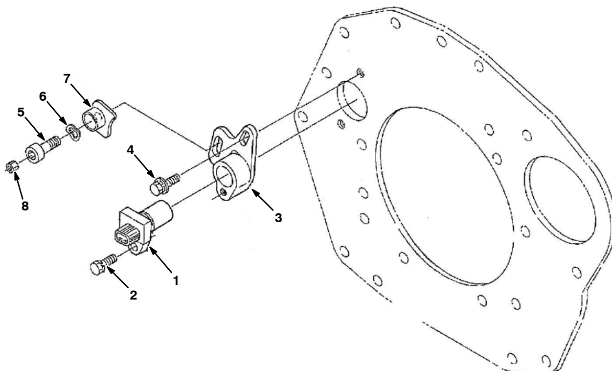
Fig. 16 - Sensor Group
