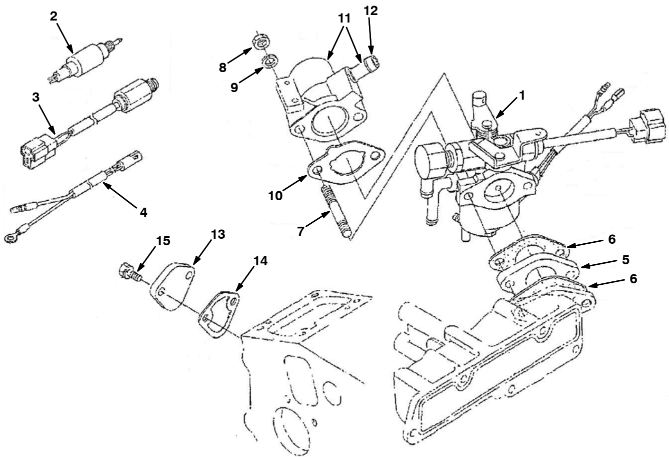
Fig. 12 - Carburetor Group
