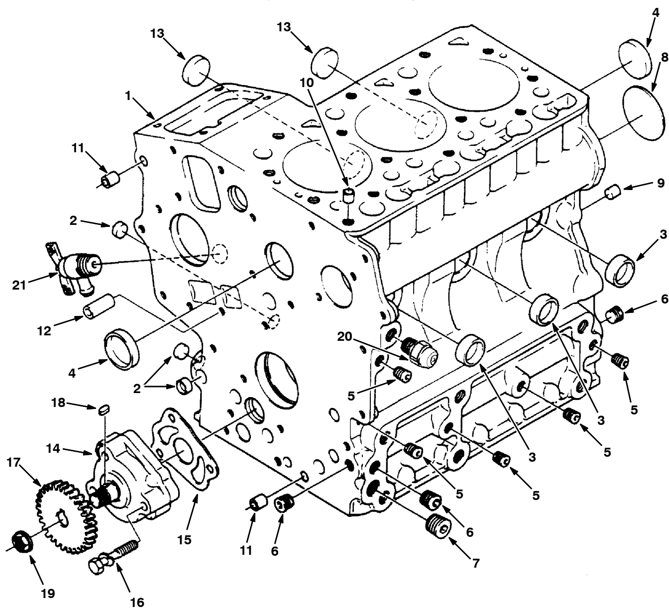
Fig. 1 - Crankcase Group
