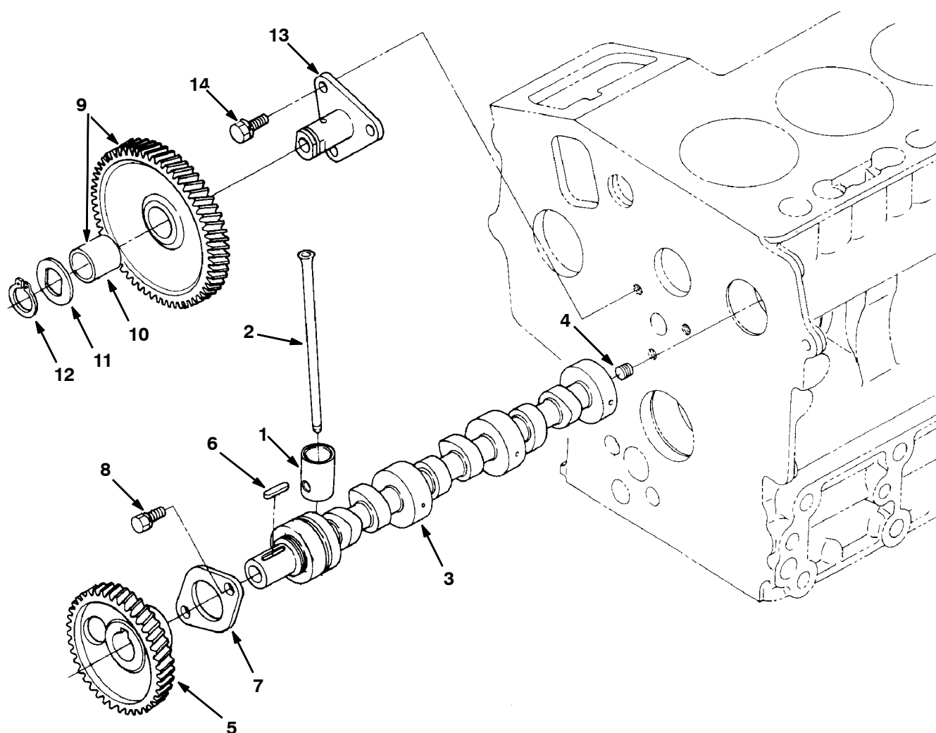
Fig. 8 - Camshaft Group
